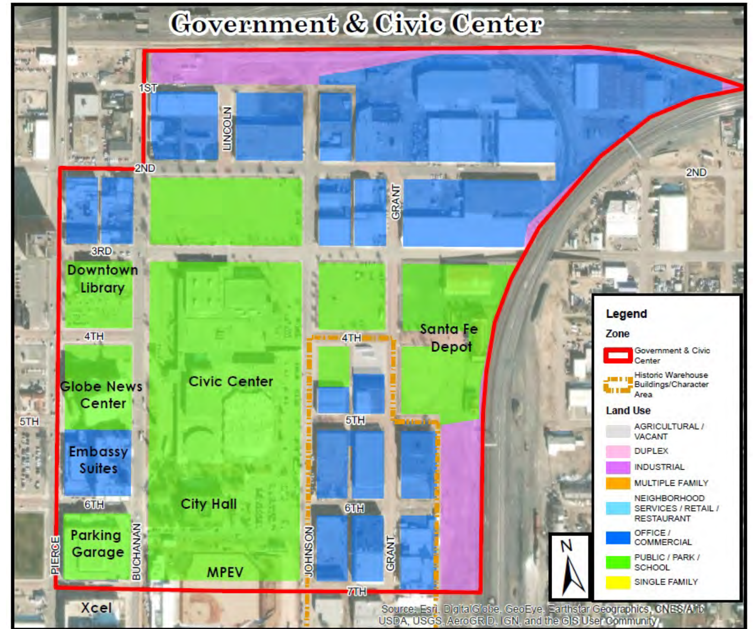
Current Land Use - 2019
