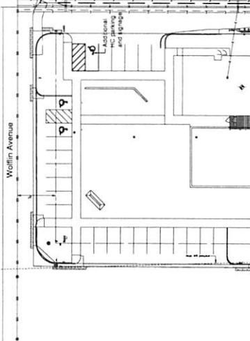
1 DETAIL - DRIVE APPROACH
