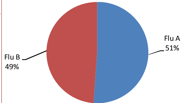
Fig. 2 Flu A & B Comparison
