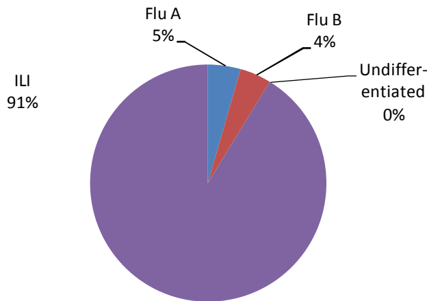
Fig. 1 Flu Testing By Percent
