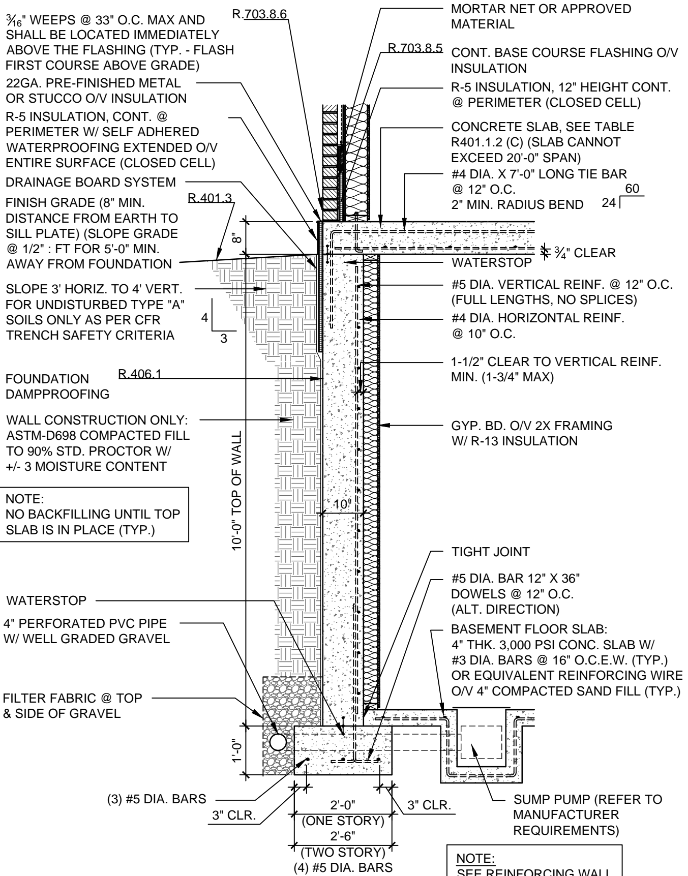
10" FORMED BASEMENT PERIMETER WALL DETAIL W/ BRICK SCALE: 1/2" = 1'-0"
